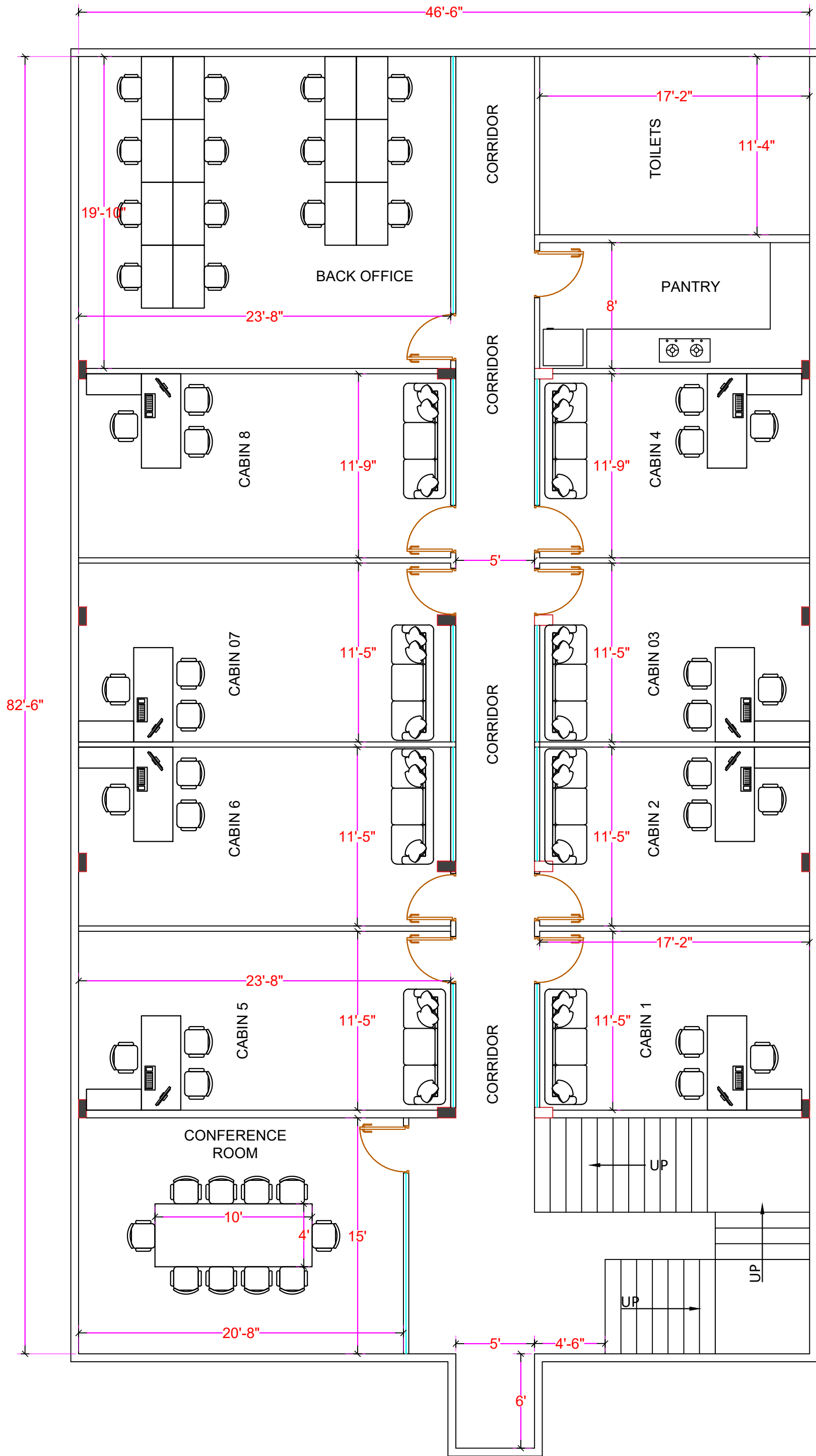
GROUND FLOOR
